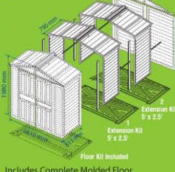
Includes Complete Molded Floor YardMate
